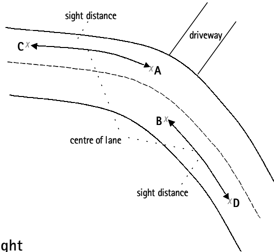
Figure 6.1: Sight distance measurement
