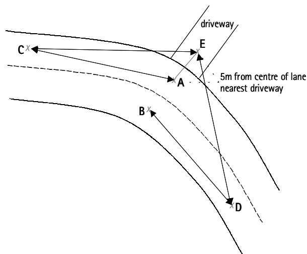
Figure 6.2: Lines of clear sight
